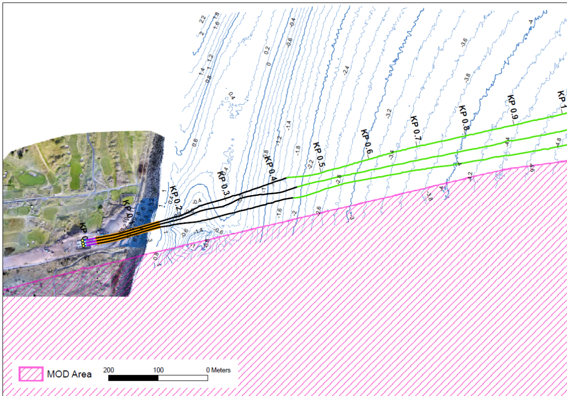
Fig 1 – Carnoustie nearshore export cable survey area.
